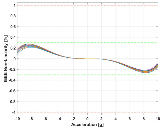
Figure 3 : Non-linearity IEEE
