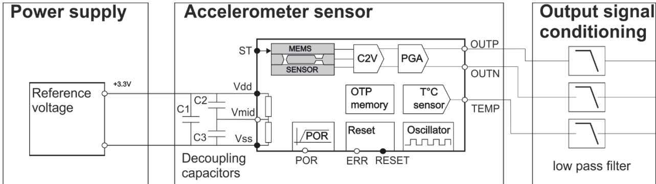
Figure 20 : Recommended Block diagram
