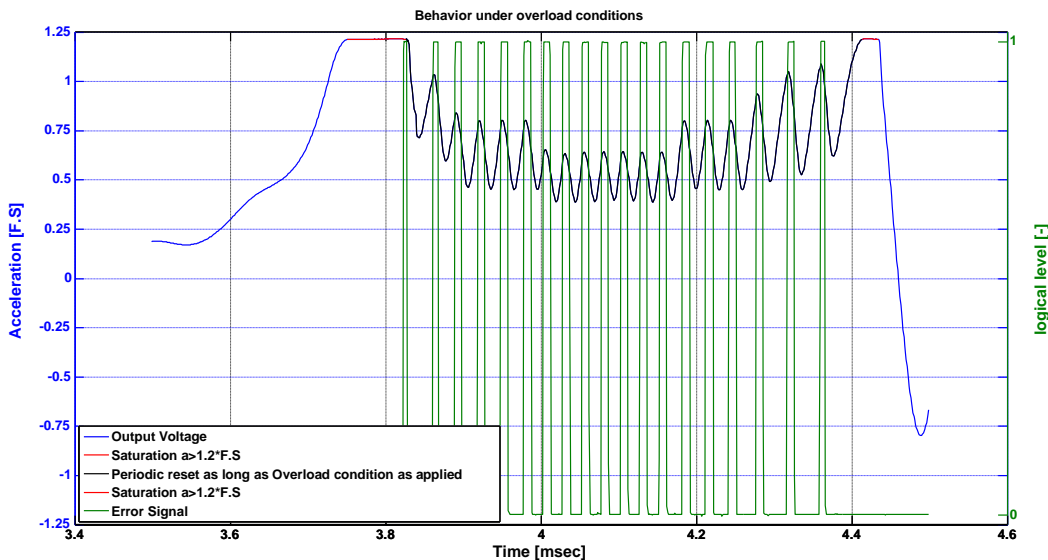
Figure 18 : Overload Behavior
