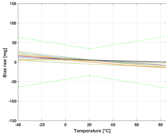
Figure 1: Raw bias
