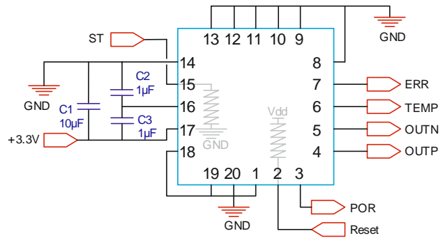
Figure 14 : Proximity circuit & internal pull-up/down
