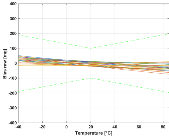
Figure 7: Raw Bias over temperature
