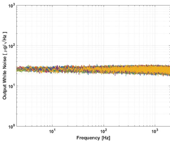
Figure 5: Typical white noise
