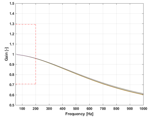
Figure 4 : Frequency response
