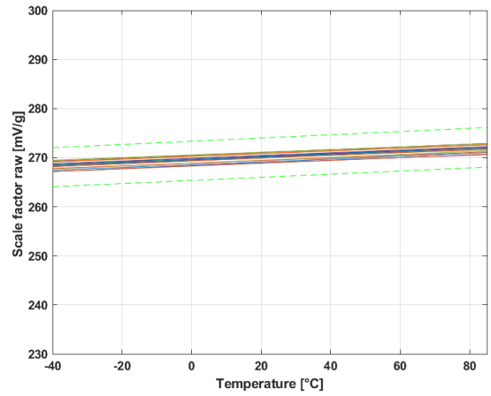
Figure 2: Raw scale factor
