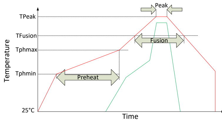
Figure 22: Soldering Temperature Profile
