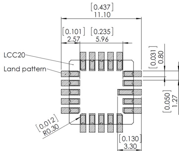
Figure 21 : LCC20 land pattern recommendation (unit are mm/[inch])
