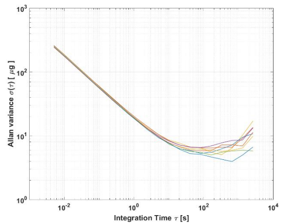
Figure 6: Allan Variance
