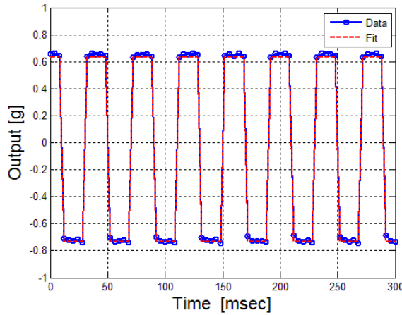
Figure 17 : Built-in Self-Test signal on the differential acceleration output (frequency: 24 Hz / amplitude 1.3 g)
