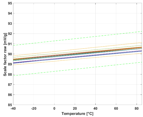
Figure 8: Raw Scale Factor over temperature
