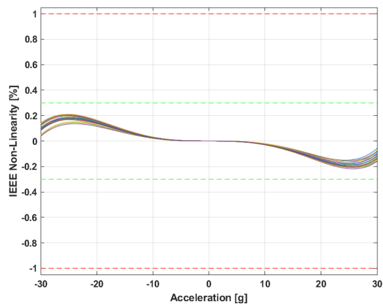
Figure 9 : Non-linearity IEEE
