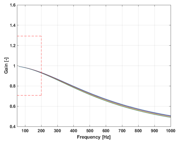
Figure 10 : Frequency response
