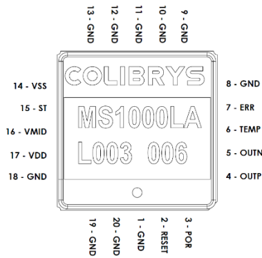
Figure 13 : Pinout top view
