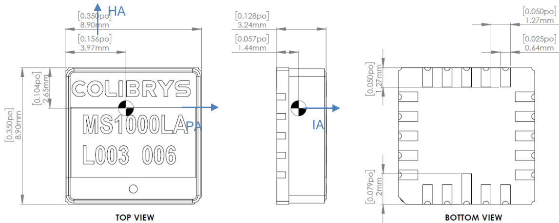
Figure 19 : Package mechanical dimension. Units are mm [inch]
