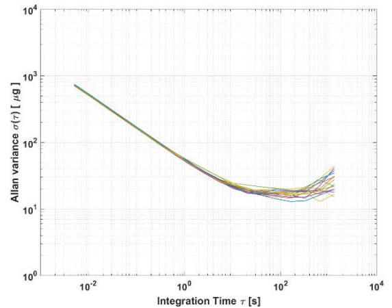
Figure 12: Allan Variance
